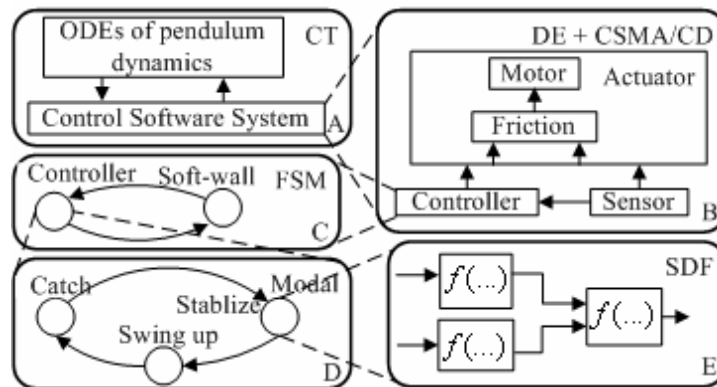
Fig. 2. Integration of runtime models in Cyveh
