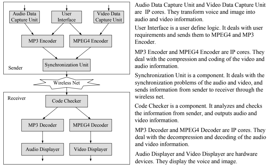
Fig. 8. The audio and video architecture design of the PDA platform
