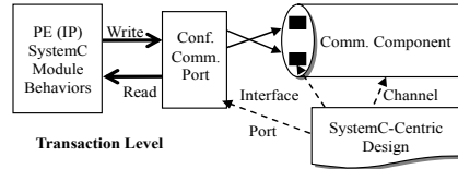
Fig. 5. SystemC-based architecture model
