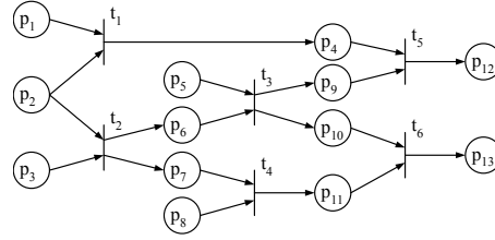
Fig. 3. The Petri net model of the example design
