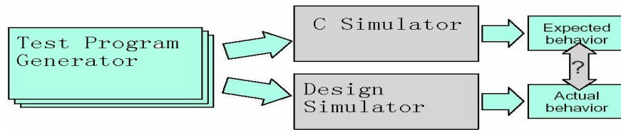
Fig. 4. The workflow of co-verification
