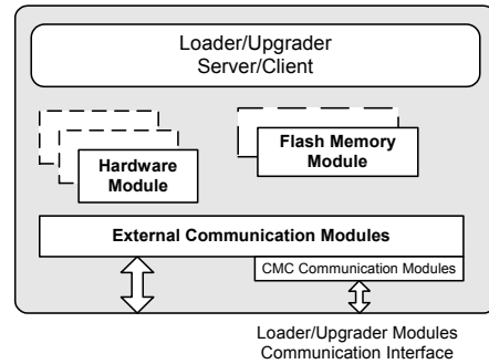
Fig. 2. Structure of the server and client modules
