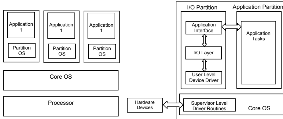
Fig. 1. vxWorks AE653 OS and Device Driver Models
