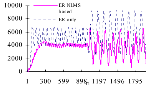
Fig. 4. Comparison of ER only and ER with NLMS
