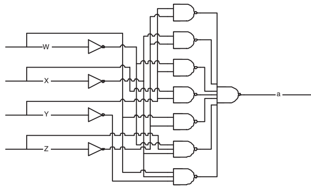
Fig. 3. Schematic Design
