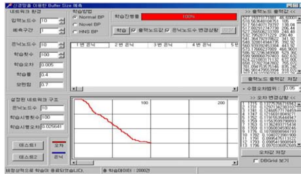
Fig. 5. The learning result on the prediction of buffer size using BP
