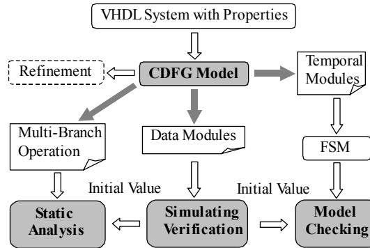
Fig. 3. Functional verification flow
