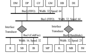
Fig. 8. Topology exploration
