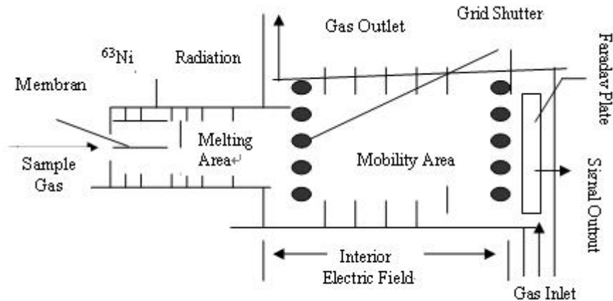
Fig.2 The Basic Structure of IMC
