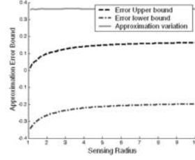
Fig. 3. Approximation error
