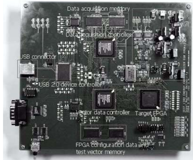
Fig. 7. SECF (SNU Energy Characterizer for FPGAs).
