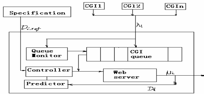
Fig. 1. The queueing model structure in embedded web server
