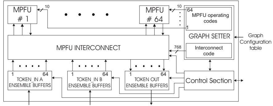
Fig. 3. Platform-Processor block scheme.
