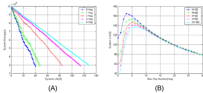
Fig. 3. Simulation results(1)
