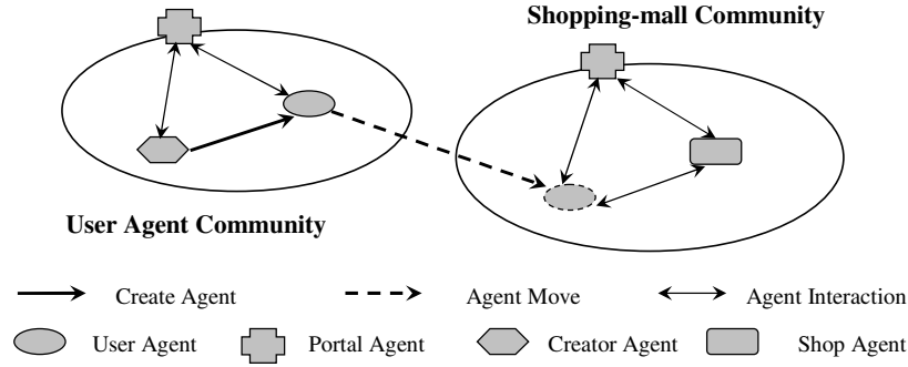
Fig. 2. An overview of the agent society
