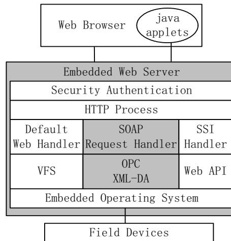
Fig. 2. Structure of OPC-EWS
