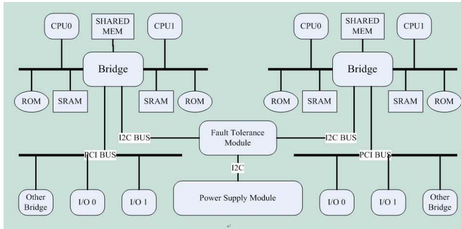
Fig. 1. The architecture of Highly-reliable Embedded Multiprocessors system
