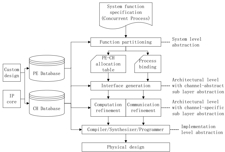
Fig. 4. Design flow
