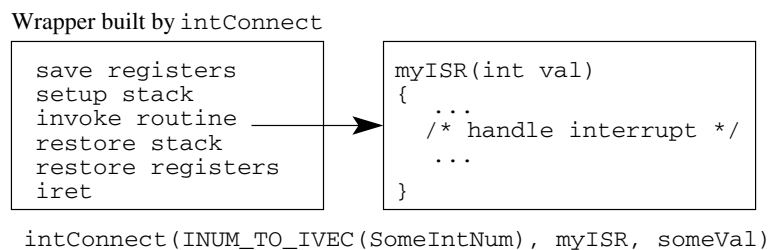
Fig. 2. Routine built by intConnect in embedded operating systems. By wrapping the myISR function, registers and stack pointers are automatically saved/restored when interrupts occur
